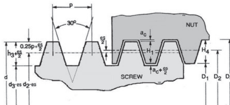
TRAPEZOIDAL THREADED NUTS BS 5346 (DIN 103) Grade 7H
